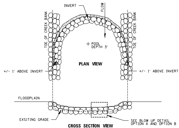
CROSS VANE DETAIL LOOKING UPSTREAM N.T.S.
