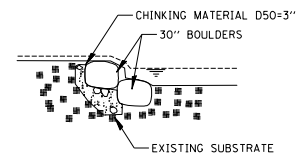
CROSS VANE TYPICAL PROFILE DETAIL
