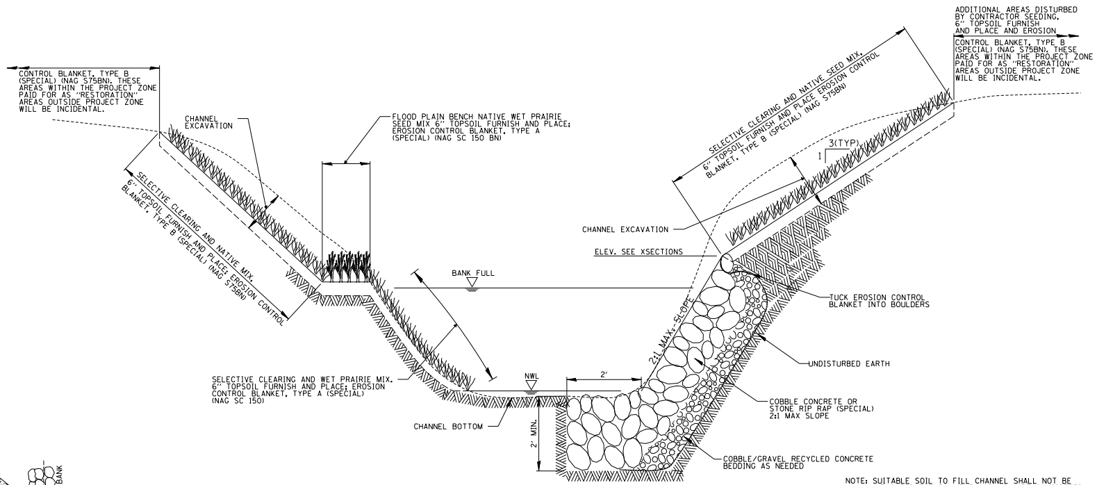
TYPICAL SECTION
